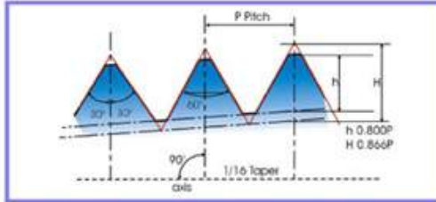
Fig. 4 (Taper) H = 0.866025 P h = 0.800000 P
