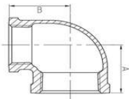
Street Elbow, 90°
