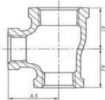
Reducing Tee
