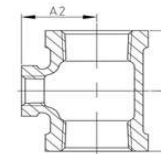
Reducing Tee
