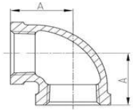
Reducing Elbow, 90°
